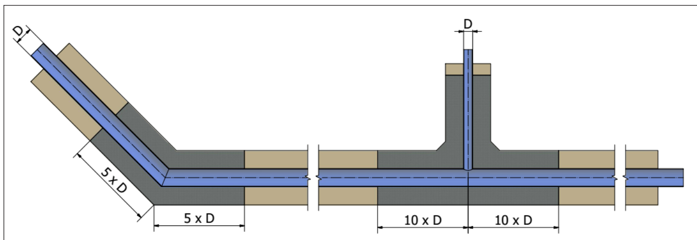
Figure 1 - Backfill with compacted friction material around bends and tees to minimize movements in buried PE pressure pipe systems
