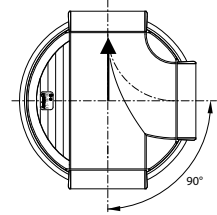
junction 90° (90°)
