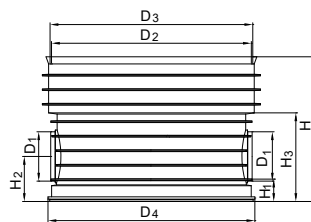
junction 90° (270°)
