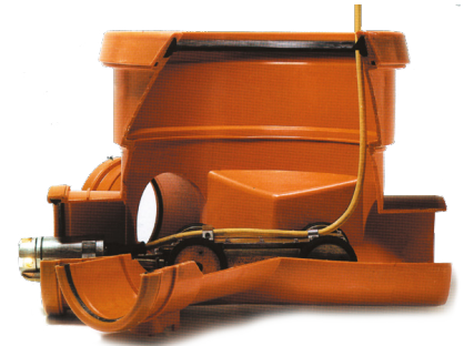
Insertion of a mobile video camera to the sewer through a PRO 400 mm chamber.
