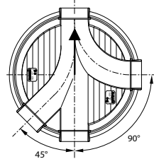
junction 45° (225°), 90° (90°)
