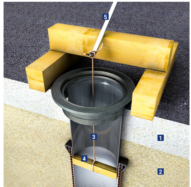
Telescope adjustment using a rope
