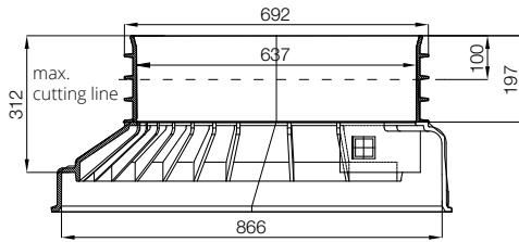
Reducer 800/630
