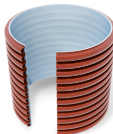
Riser pipe 400 mm PP-B DW SN 8 kN/m 2
