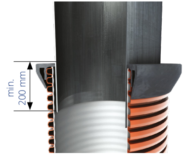
Correct installation of the telescopic pipe in the riser pipe of the chamber.
