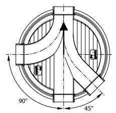
junction 90° (270°), 45°(135°)
