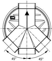
junction 45° (225°), 45° (135°)
