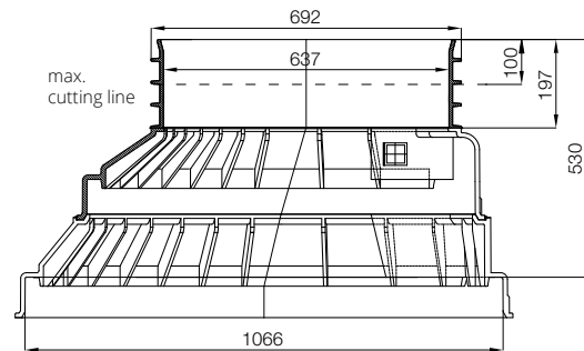
Reducer 1000/630
