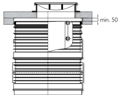
Chamber with a concrete slab
